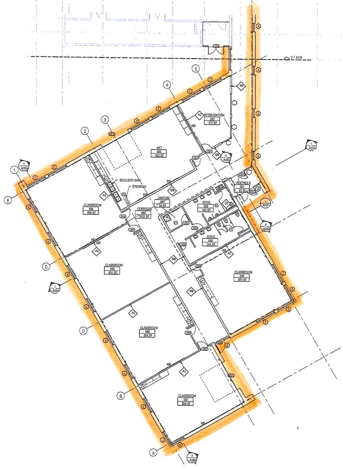
1 Floor Plan - Classroom Addition A110 1/8" = 1'-0"
